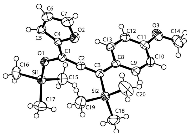
Figure 2. Molecular structure of allene 5h in the solid state. Thermal displacement ellipsoids are drawn at 50% probability. Selected bond lengths and angles: C1–O1 1.380(3), O1–Si1 1.665(2), C1–C2 1.316(4), C2–C3 1.322(4), C3–Si2 1.898(3) Å; C1–O1–Si1 128.6(2), C1–C2–C3 172.6(3), C2–C3–Si2 115.0(2)°.
