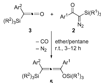
Scheme 5. Synthesis of 3-silyl-1-silyloxyallenes 5 .
