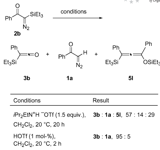
Scheme 2. Acid-induced transformation of 2b .
