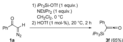
Scheme 3. One-pot synthesis of silyl ketene 3f by diazo ketone silylation/acid-induced Wolff rearrangement.
