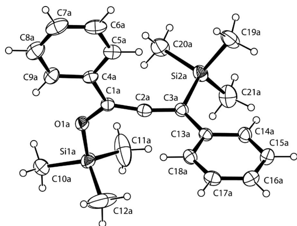
Figure 1. Molecular structure of allene 5a in the solid state. Thermal displacement ellipsoids are drawn at 30% probability. Selected bond lengths and angles (only one of the two molecules in the asymmetric unit is shown above; data for the second molecule are enclosed in brackets): C1–O1 1.375(3) [1.383(3)], O1–Si1 1.655(2) [1.662(2)], C1–C2 1.320(3) [1.320(3)], C2–C3 1.318(3) [1.318(3)], C3–Si2 1.893(2) [1.899(2)] Å; C1–O1–Si1 129.9(2) [129.0(1)], C1–C2–C3 170.1(2) [172.2(2)], C2–C3–Si2 114.1(2) [114.8(2)]°; torsion angles: C2–C1–C4–C5 9.3(3) [4.9(3)], C2–C3–C13–C18 –5.2(3) [173.9(3)], C2–C1–O1–Si1 10.3(3) [19.1(3)]°.
