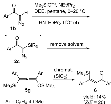
Scheme 4. Transformation of silyldiazo ketone 2c during workup.
