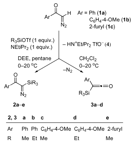
Scheme 1. Synthesis of silyldiazo ketones 2 and silyl ketenes 3 .
