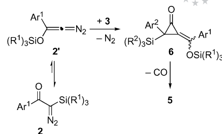
Scheme 6. Proposed mechanism for the formation of allenes 5 .
